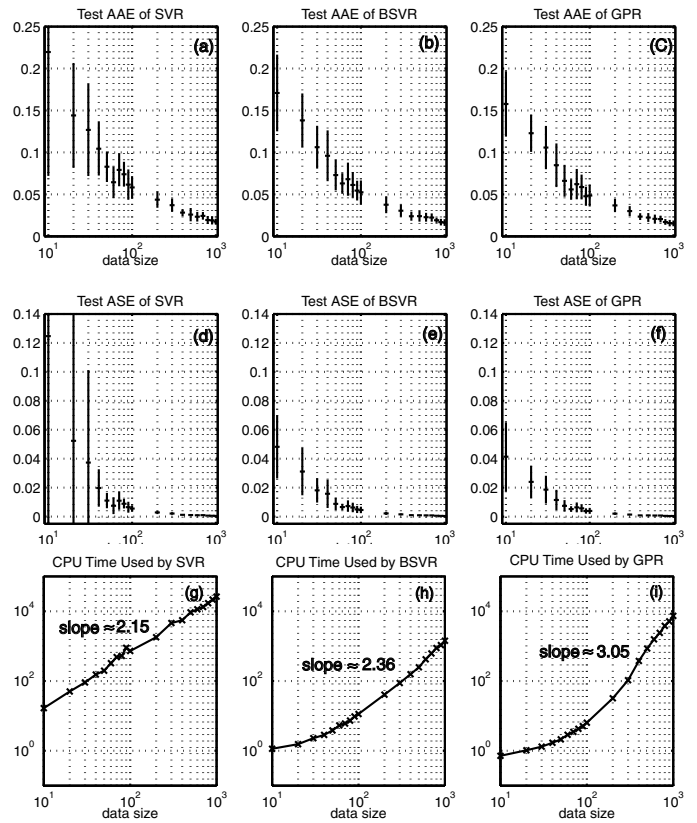
Fig. 4. SVR, BSVR and GPR on the simulated sinc data at different training data size. The results of AAE and ASE are presented in the graph (a)~(f) respectively. BSVR and GPR used evidence maximization to choose optimal hyperparameters, while five-fold cross validation was used for SVR. The position of cross denotes the average values over the 20 repetitions, and the vertical line indicates the standard deviation. In the graph (g)~(i), we present the total CPU time in seconds consumed by these three approaches in training and test at different data sizes.
